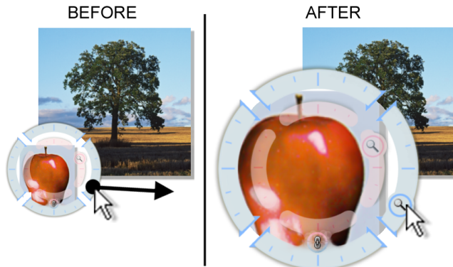
Figure 6. Resizing the telescope – no additional content from the target is revealed or lost. (a) before operation. (b) after operation.
